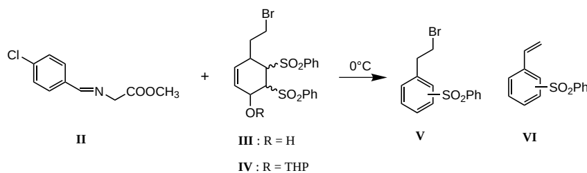
Scheme 3. Tentative attempts to alkylate the glycine Schiff base II .
