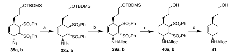
Scheme 10. a) \text{H}_2 (5 bars), \text{Pd}(5\%)/\text{CaCO}_3\text{-Pb}(3.5\%) , \text{THF}/i\text{PrOH} (1:1), RT. b) \text{ClCO}_2\text{AlI} , \text{EtOH} , \text{NaHCO}_3 , sonication, RT, 76% from 35 . c) \text{MeOH} , \text{H}^+ , RT, 86%. d) \text{Na}(\text{Hg}) , \text{MeOH} , \text{KH}_2\text{PO}_4 , RT, 74%.
