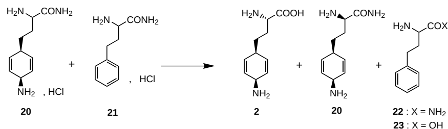
Scheme 7. Conversion of D,L-amino acid amide 20 into L-amino acid 2 and D-amino acid amide 20 with the aid of immobilised pronase in a phosphate buffer (pH 9.6) at 37 °C.
