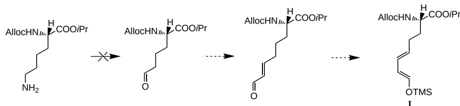
Scheme 2. Unsuccessful attempts to prepare Diels–Alder diene 1 .
