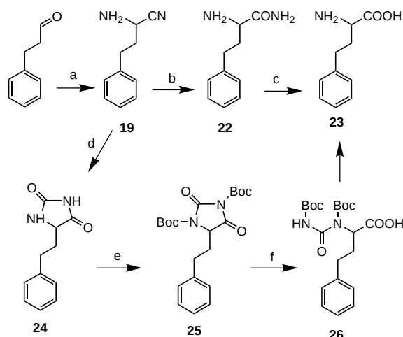
Scheme 6. a) TMS-CN, ZnI 2 , CH 2 Cl 2 , RT; NH 3 , MeOH, 73%. b) H 2 O 2 , NaOH, MeOH, RT, 76%. c) NaOH or LiOH or Na 2 O 2 , H 2 O, RT. d) (NH 4 ) 2 CO 3 , H 2 O, MeOH, 50 °C, 62%. e) Boc 2 O, DMAP, THF, RT, 65%. f) LiOH, THF/H 2 O (5:1), RT, 92%.
