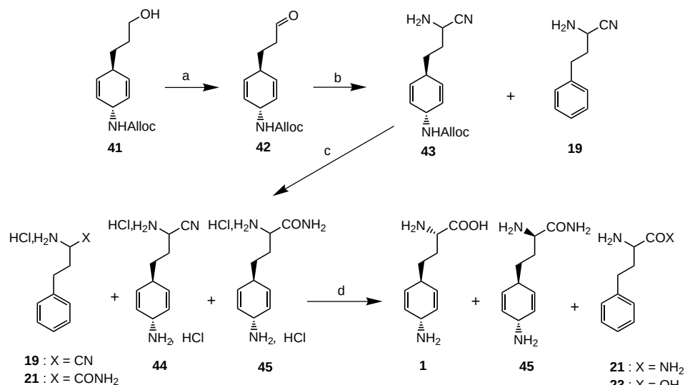
Scheme 11. a) (\text{COCl})_2 , \text{DMSO} , \text{CH}_2\text{Cl}_2 , -60^\circ\text{C} ; \text{NEt}_3 , -20^\circ\text{C} , quantitative yield. b) \text{TMS-CN} , \text{ZnI}_2 , \text{CH}_2\text{Cl}_2 , RT; \text{NH}_3 , \text{MeOH} , 51%. c) \text{Pd}(\text{PPh}_3)_4 , \text{PhSiH}_3 , \text{CH}_2\text{Cl}_2 , RT; \text{HCl} , 85%. d) immobilised pronase, phosphate buffer, pH 9.6, 37^\circ\text{C} , 1 : 20%, 45 : 20%.
