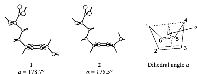
Figure 1. Modeling of compounds 1 and 2 by AM1 semiempirical methods. The dihedral angle \alpha is defined by the intersection of the (C1, C2, C3, C4) and the (C1, C6, C5, C4) planes.
