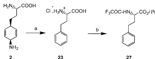
Scheme 8. a) 3 N HCl, reflux. b) 2 N i PrOH/HCl, 100 °C; (CF 3 CO) 2 O, CH 2 Cl 2 , RT. The same procedure was used for the derivatisation of 20 .
