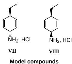
Model compounds
