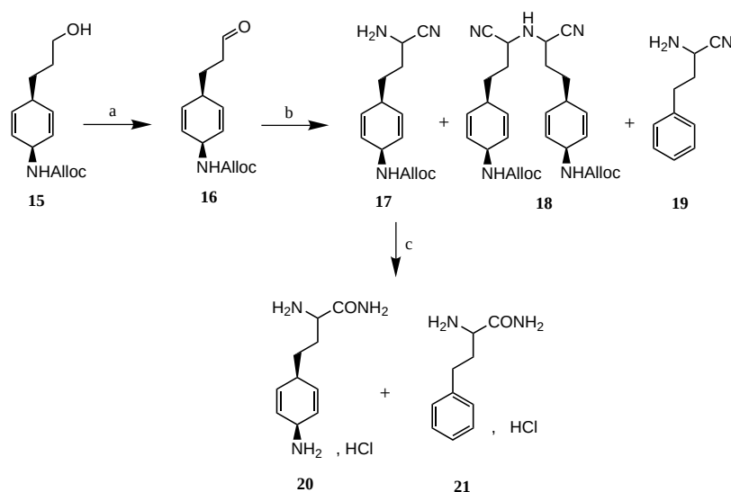
Scheme 5. a) (COCl) 2 , DMSO, CH 2 Cl 2 , –60 °C; NEt 3 , –20 °C, 95%. b) TMS–CN, ZnI 2 , CH 2 Cl 2 , RT; NH 3 , MeOH, 74%. c) Pd(PPh 3 ) 4 , PhSiH 3 , CH 2 Cl 2 , RT; HCl, 60%.
